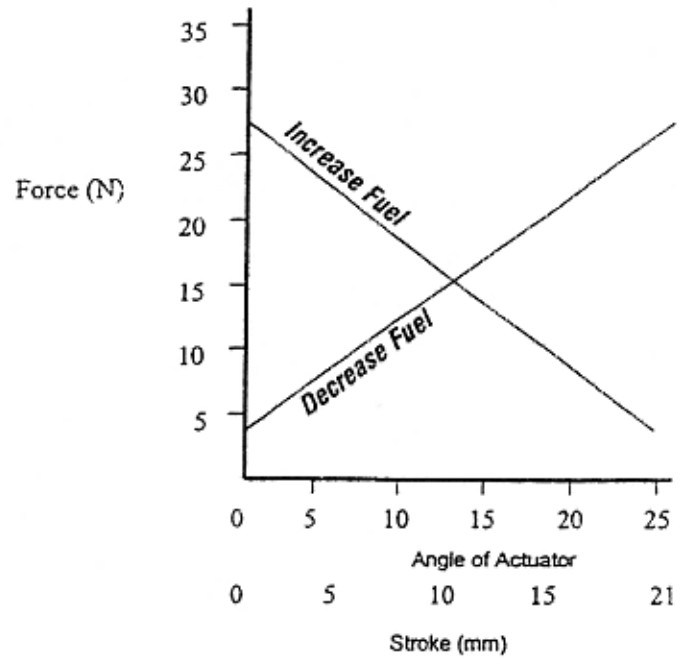
Figure 1 ACE175 Fuel Rack Force vs. Stroke
