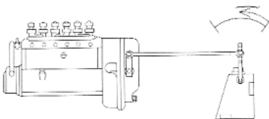
Fuel Control Lever At Mid Fuel Position DIAGRAM 3
