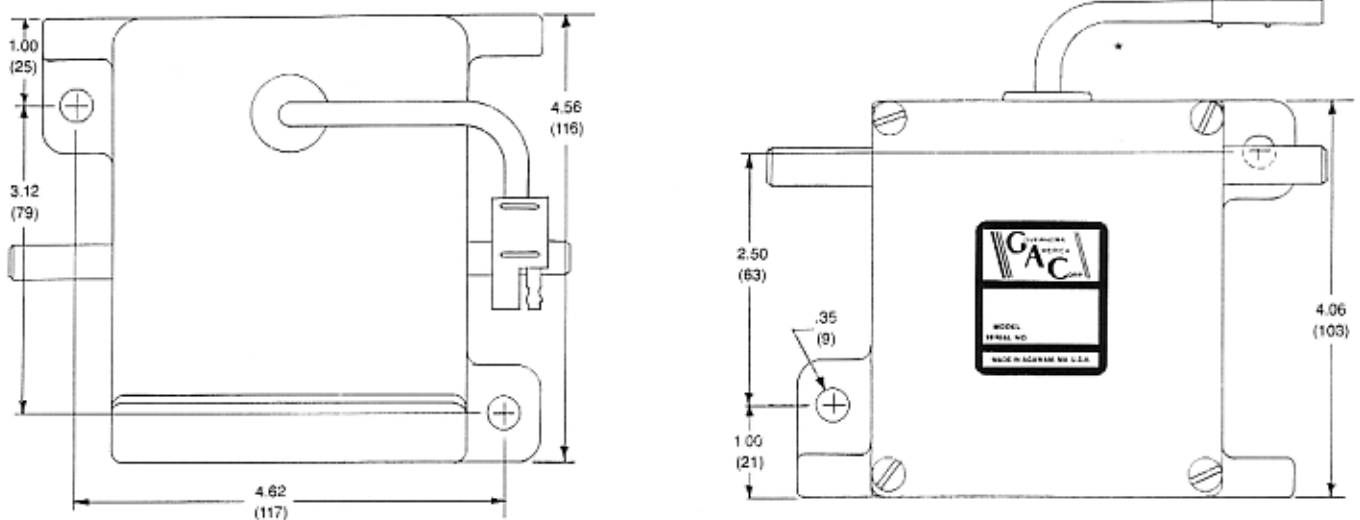
ADB and ADC Actuator Outline Dimensions
